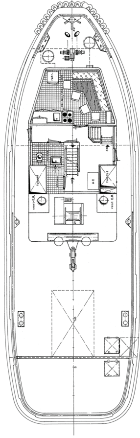
Main deck
