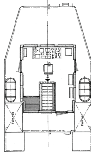
Wheelhouse
