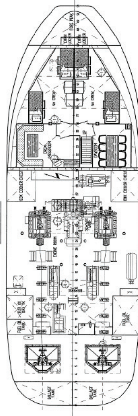
LOWER DECK
