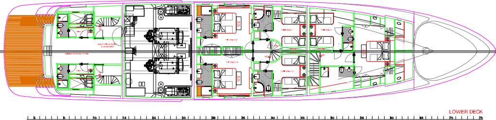
LOWER DECK
