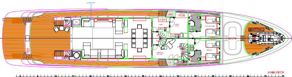
MAIN DECK
