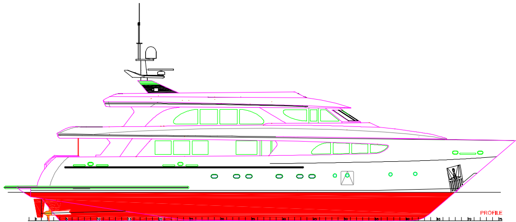
PROFILE
