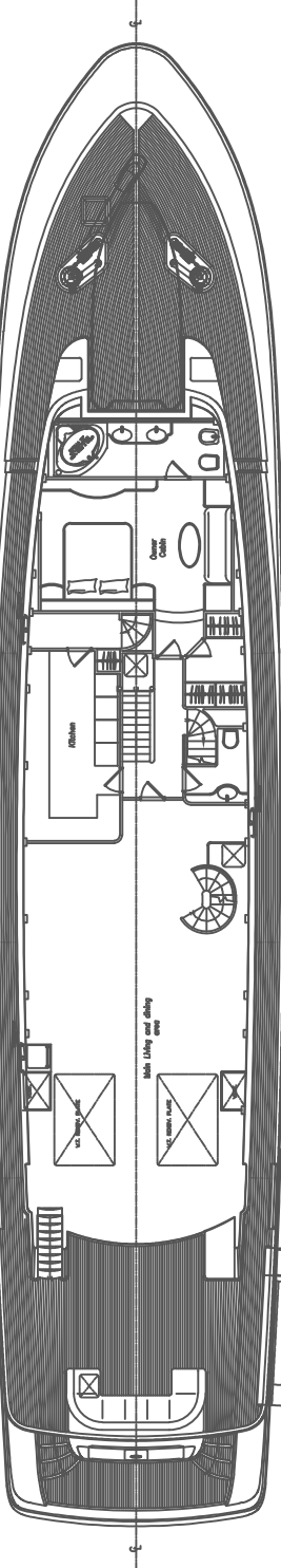
Plan View Main Deck
